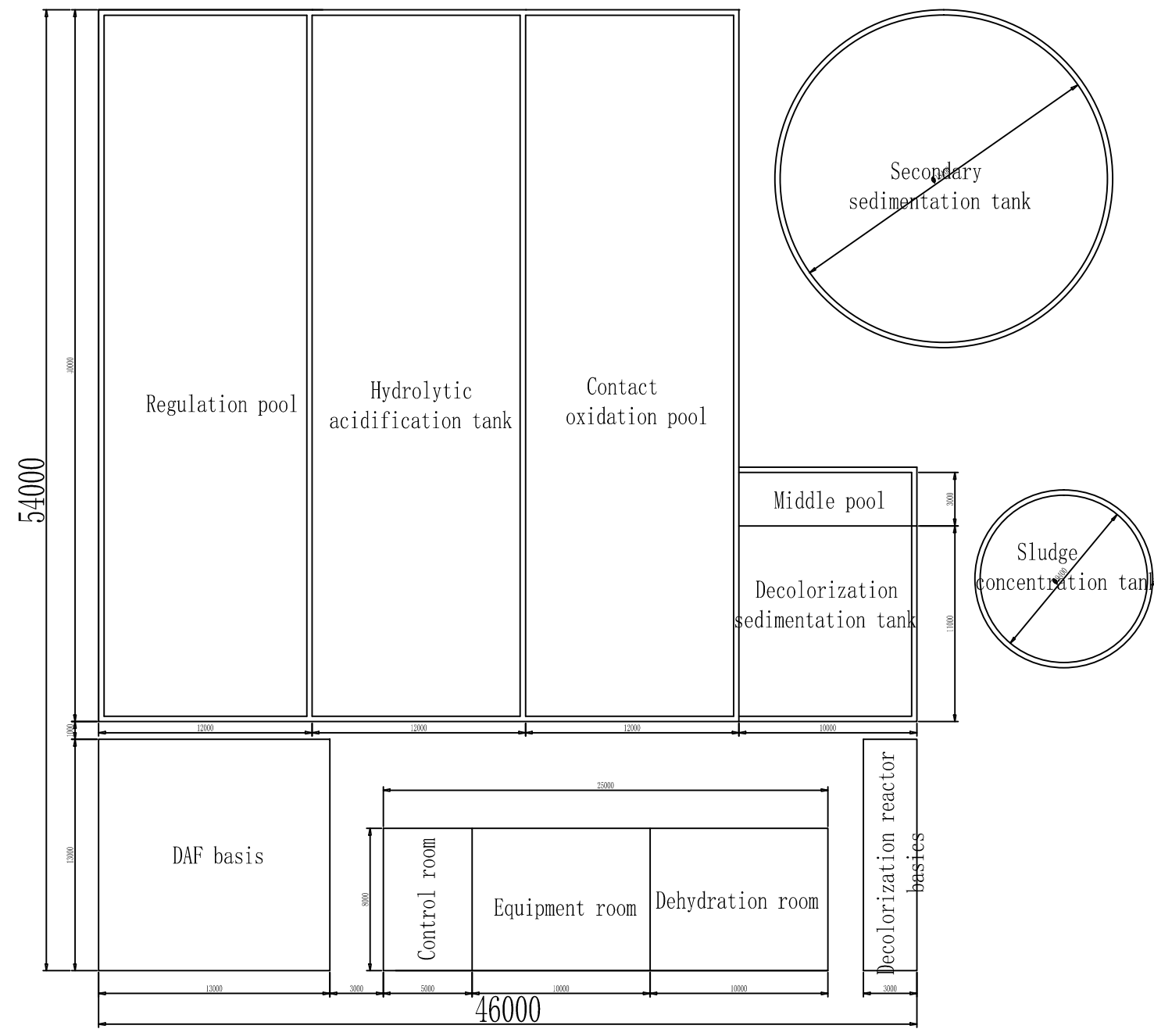
Layout plan of textile wastewater treatment
