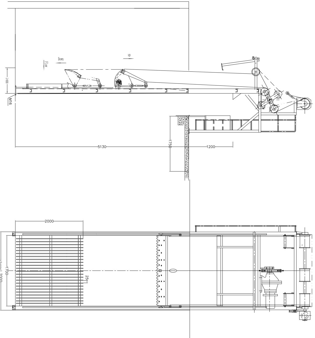
cable operated grab screen(03 cables with rake)
